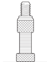
fig. 22c Woods/Dunlop valve
