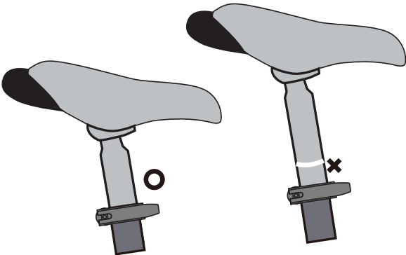
FIGURE 3 Insert into frame Minimum insertion line must be inside frame
